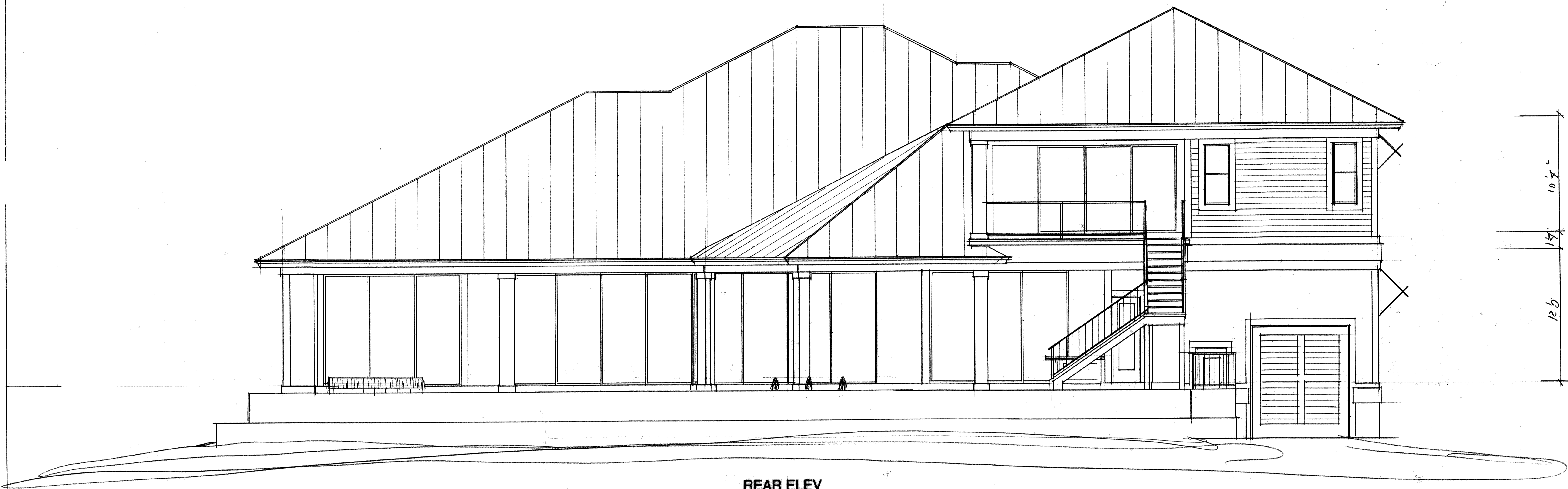
REAR ELEV
