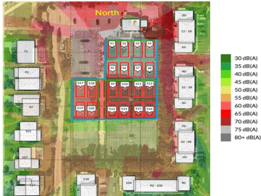
Figure 12: Noise Map, L-Shaped Expansion with 12-Foot-High Barriers to the East, West and South
