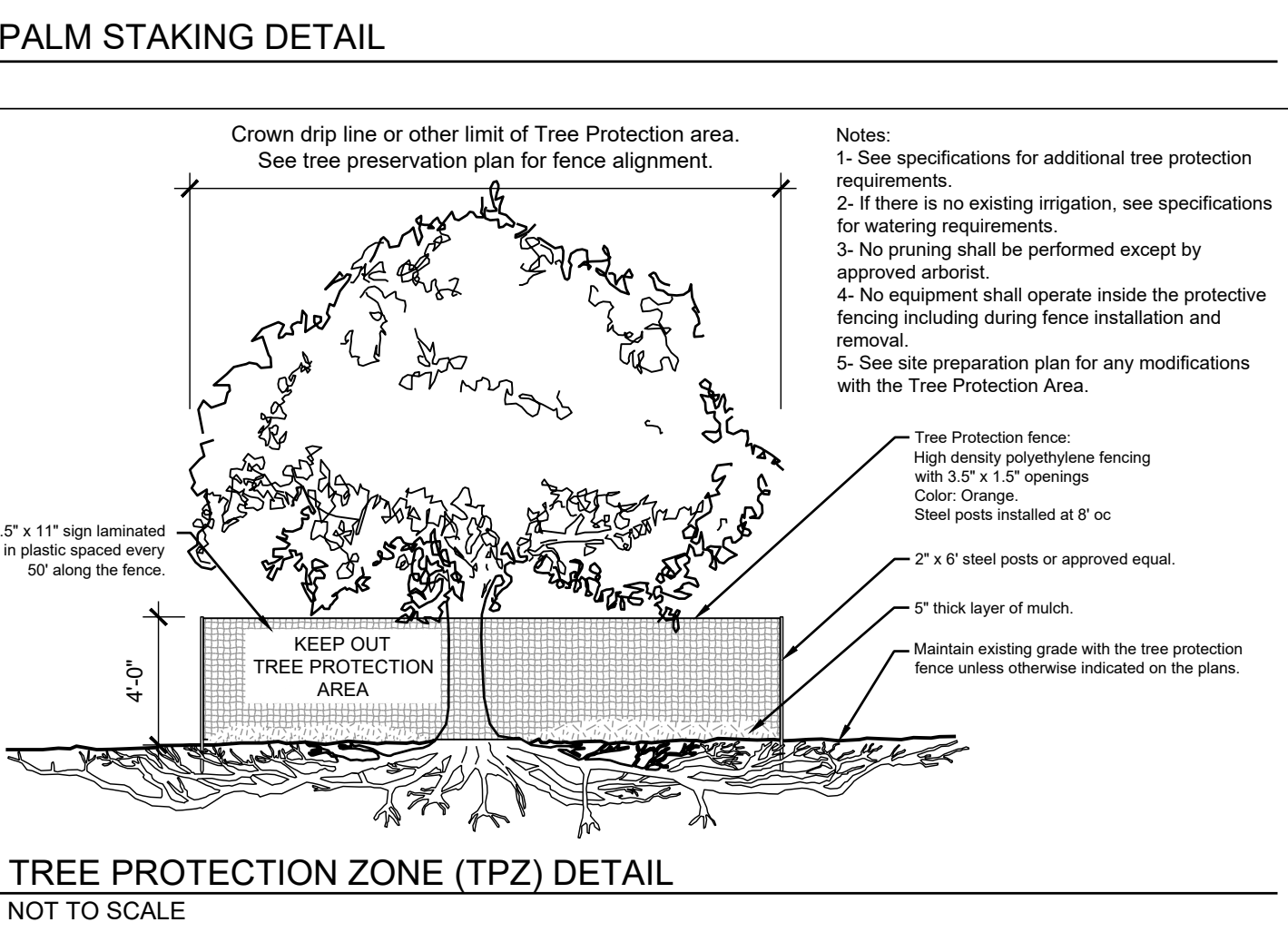
TREE PROTECTION ZONE (TPZ) DETAIL
