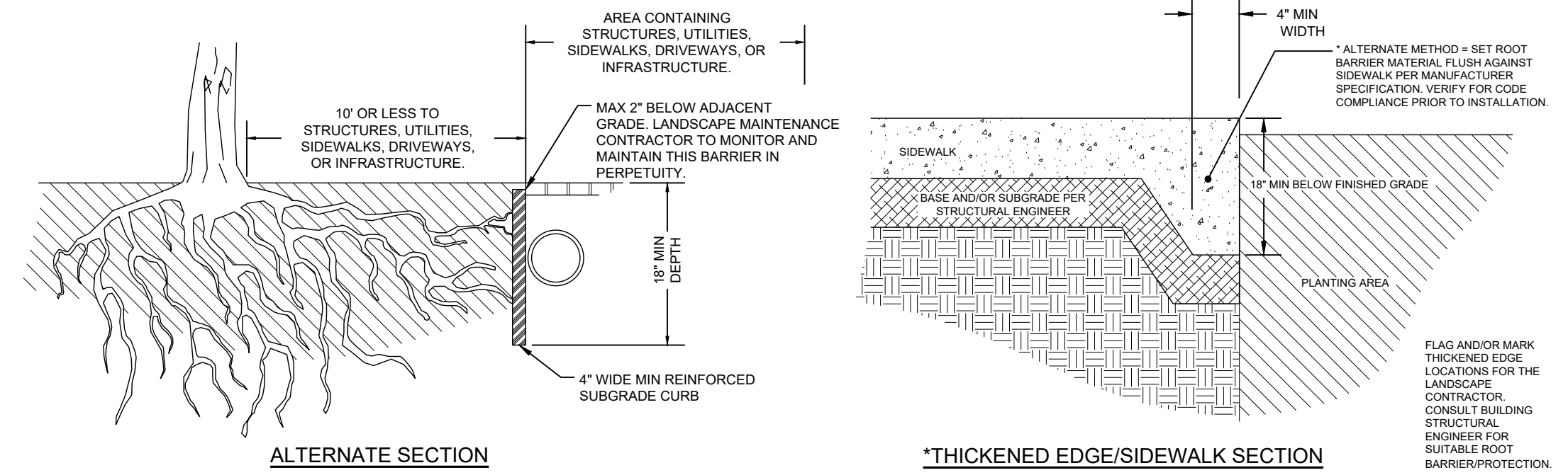
REQUIRED: ROOT BARRIER DETAIL
