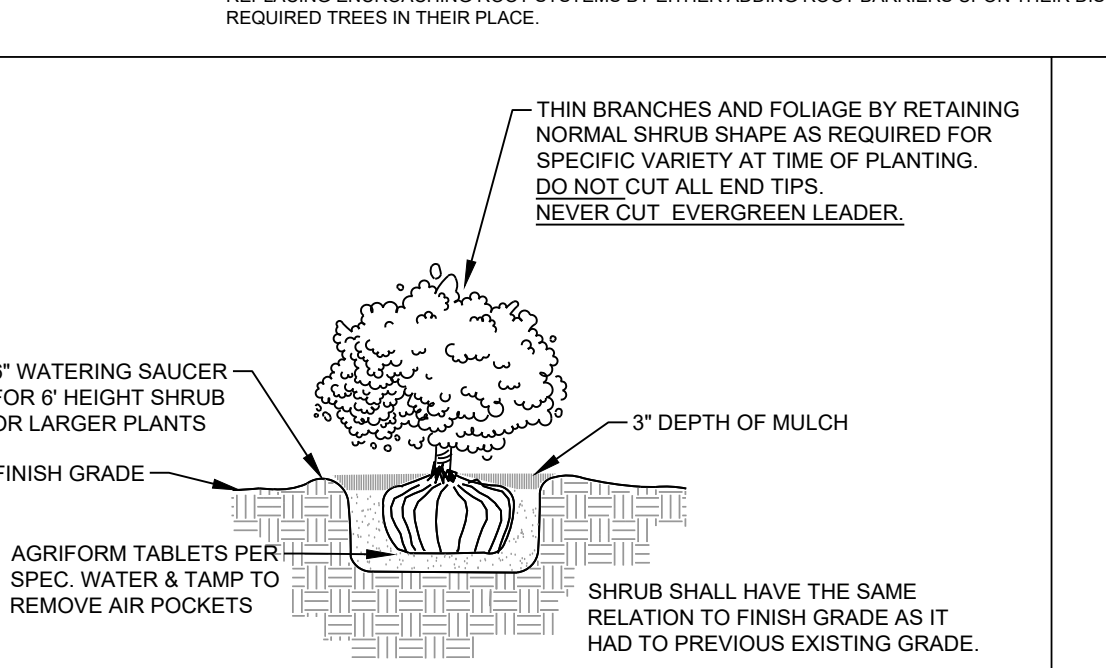
LARGE SHRUB PLANTING DETAIL
